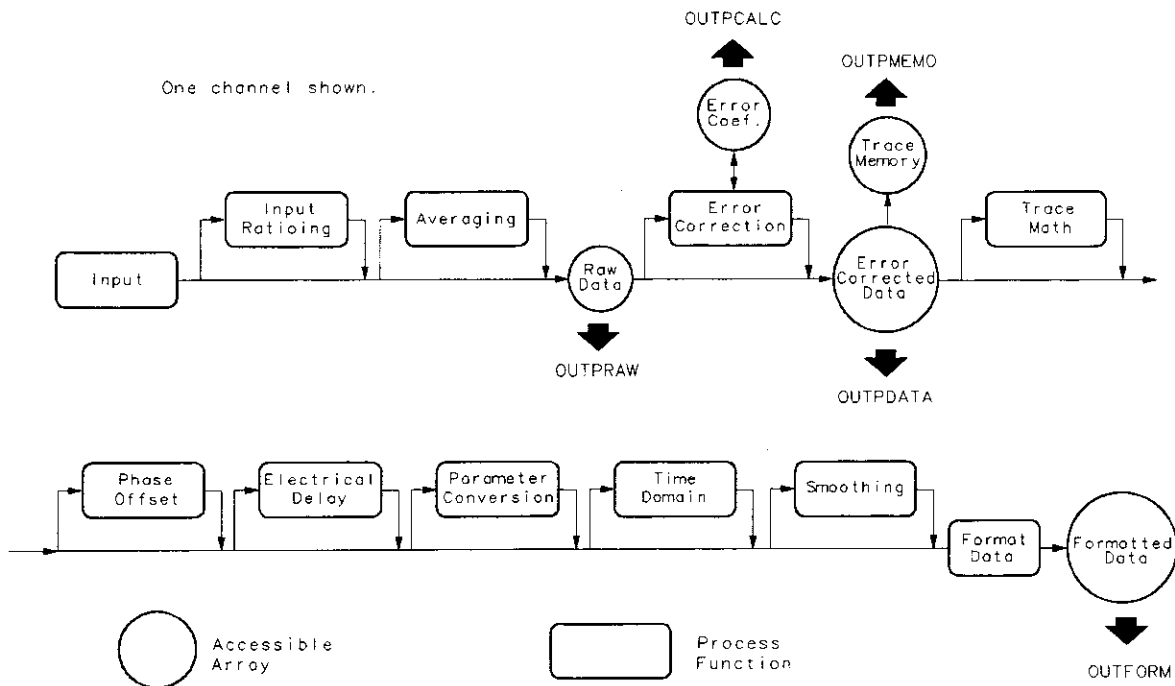
Figure 2-3. The Data-Processing Chain
