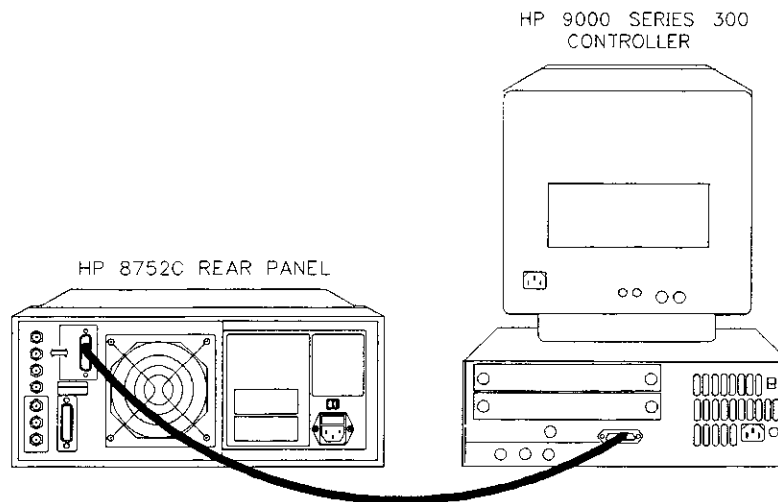
Figure 3-1. The HP 8752C Network Analyzer System with Controller
